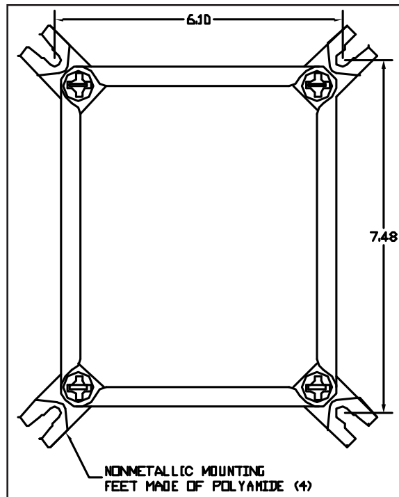
BACK OF HOUSING SHOWING MOUNTING FEET
